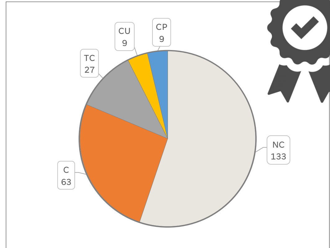
SNOMED CT
